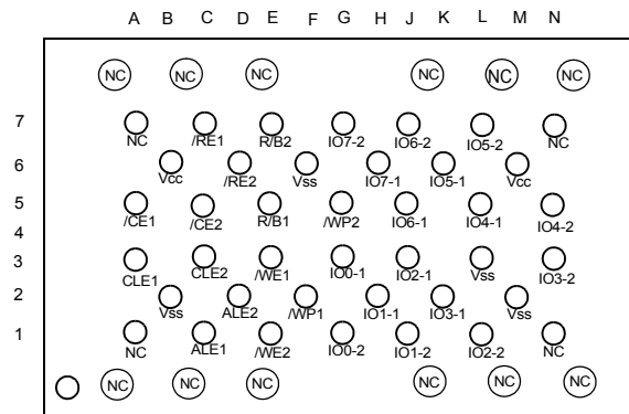
K9K8G08U1M-ICB0/IIB0
